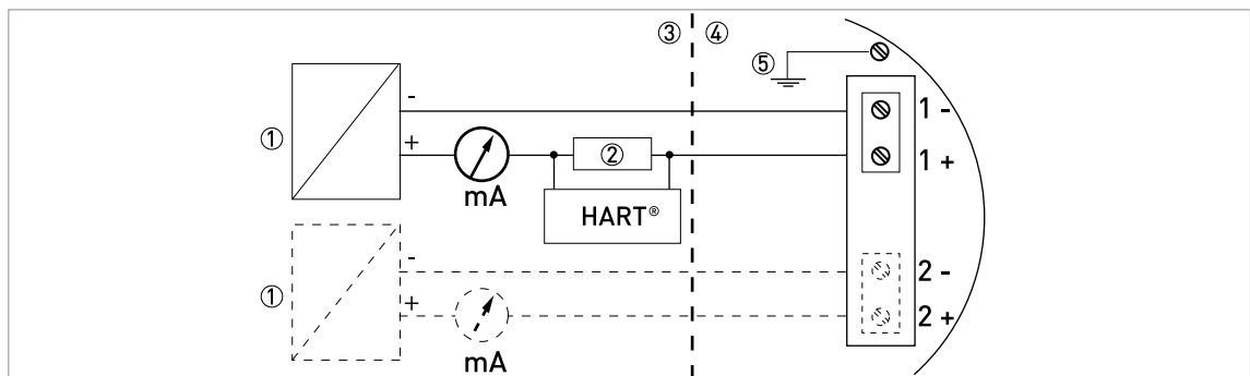
Figure 3-6: Electrical schema for Ex nA-approved equipment
