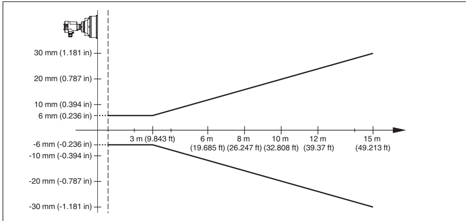
Fig. 25: Meetafwijking OPTISOUND 3030 C
