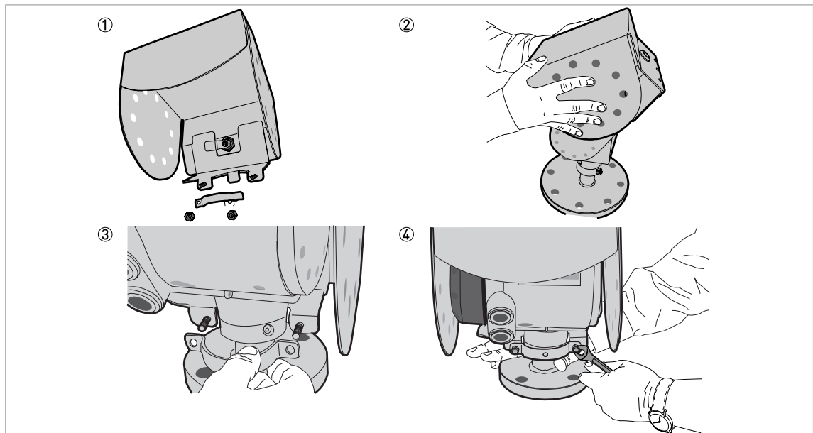
Figure 2-25: Installation of the weather protection
