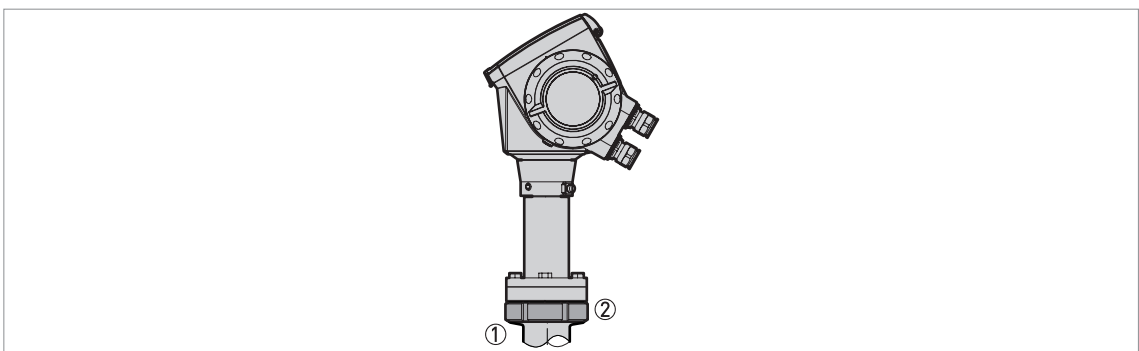
Figure 2-19: DIN 11851 connection
