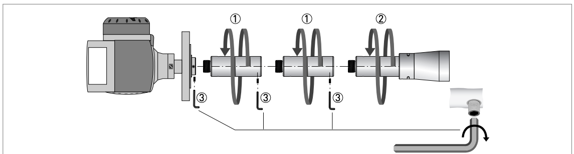
Figure 2-22: Horn antenna - how to attach antenna extensions
