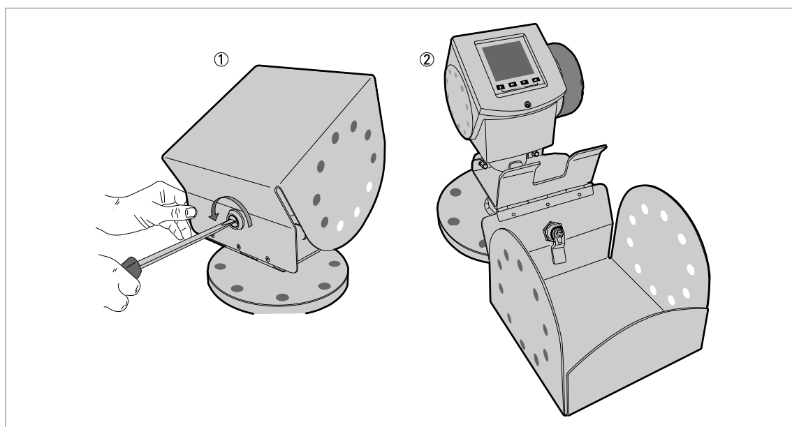
Figure 2-26: How to open the weather protection
