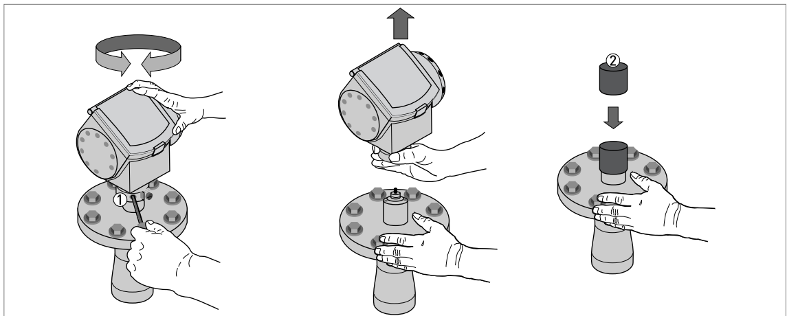
Figure 2-24: How to turn or remove the signal converter
