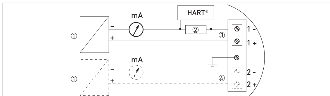
Figure 3-2: Electrical connections for non-Ex devices (standard software)
