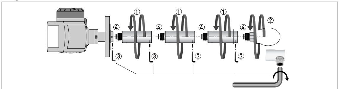
Figure 2-23: Drop antenna - how to attach antenna extensions
