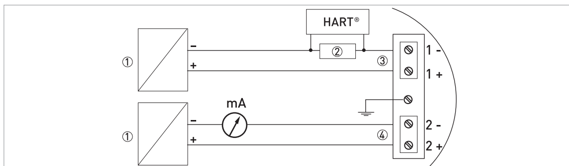
Figure 3-3: Electrical connections for non-Ex devices (fast motion software option)
