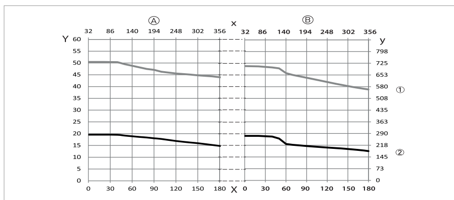
Figure 6-7: Pressure derating; ANSI B16.5
