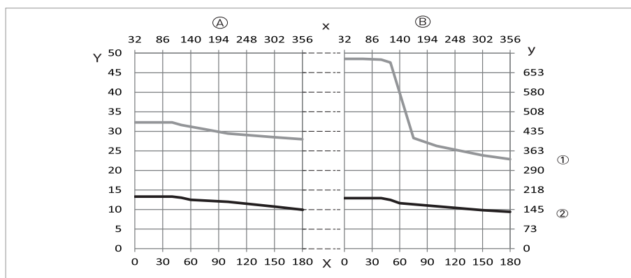
Figure 6-8: Pressure derating; JIS B2220
