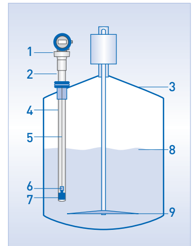
1. OPTIFLEX 2200 C 2. HT extension 3. Tank 4. Stilling well 5. Cable probe 6. Counterweight 7. Centering piece 8. Level of medium 9. Agitator
