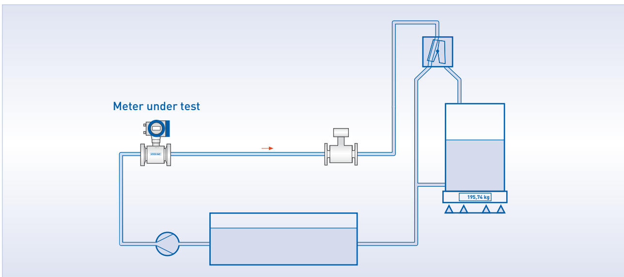
Figure 1.4: Gravimetric calibration rig
