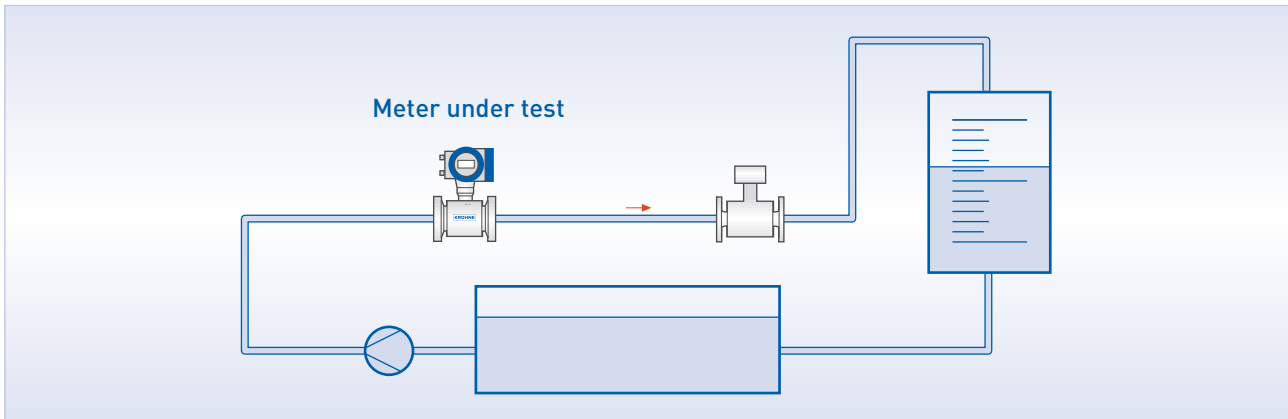
Figure 1.3: Volumetric calibration rig
