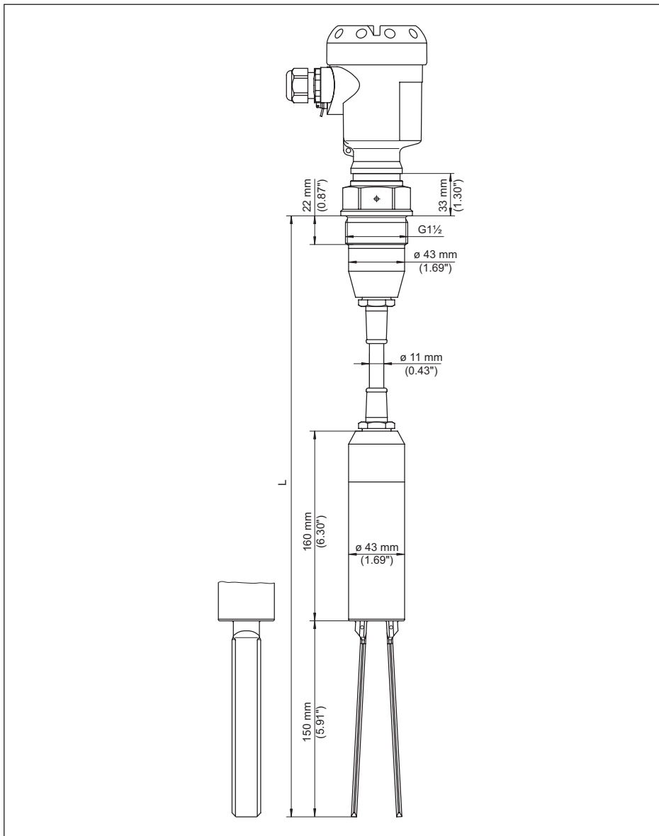
Fig. 16: OPTISWITCH 3200 C, threaded version G1½ (DIN ISO 228/1)
