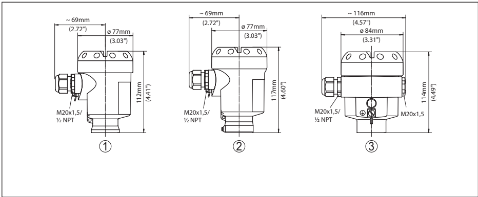
Fig. 15: Housing versions
