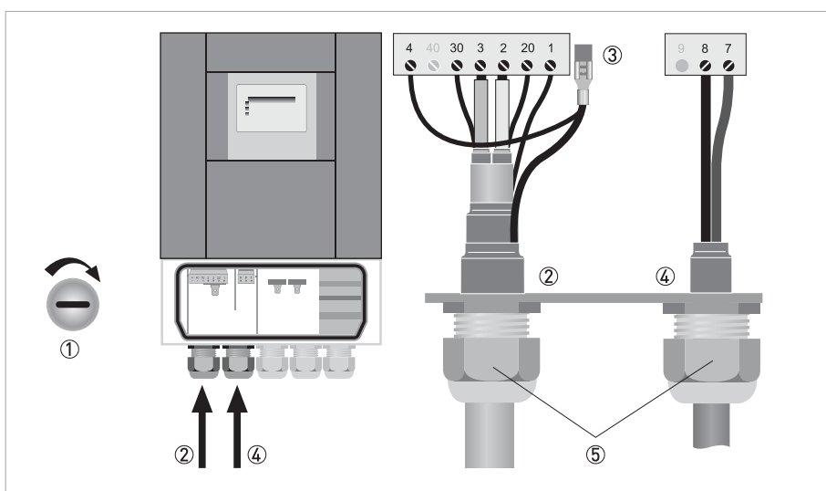
Figure 4-3: Electrical connection of the signal and the field current cables
