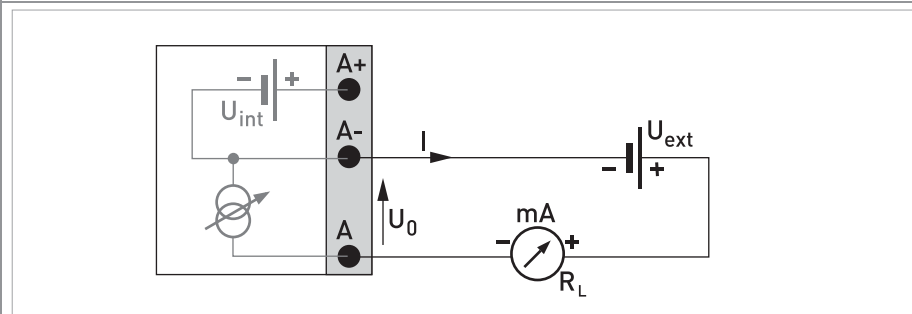
4-20mA, passive mode, grounded (external supply)
