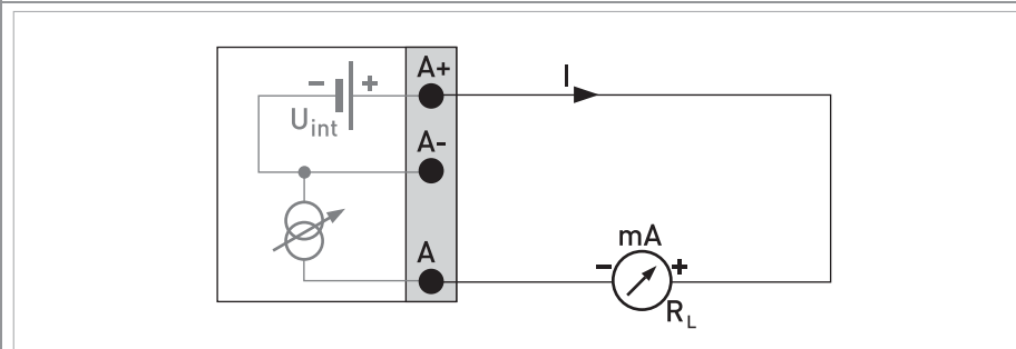
4-20mA, active mode (internal supply)
