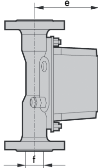
M9 Side view
