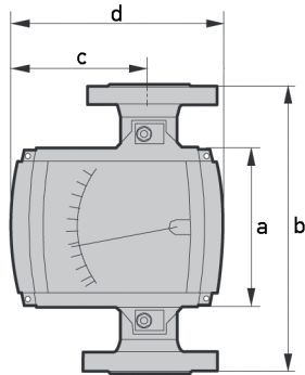
M9 Front view
