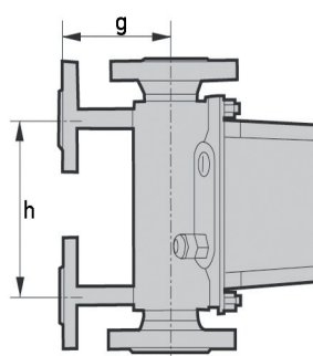
M9 with heating
